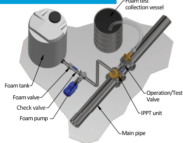
Example installation with integrated IPPT system
